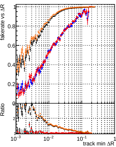
Fake rate vs \Delta R (track, jet) DQM original4 DQM testIMKFit_initialStepReso DQM testIMKFit_initialStepReso_testSorting
