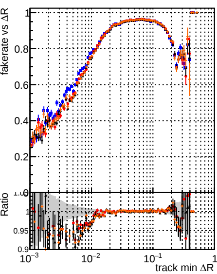
Fake rate vs \Delta R(\text{track, jet}) Legend: DOM original, test, fit, initialStepReso, testIMKFit, initialStepReso, testIMKFit, initialStepReso, testSorting
