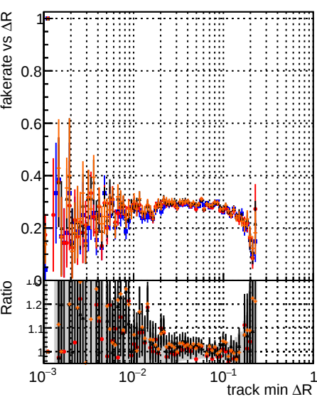
Legend: DOM original4 DOM testIMKFit_initialStepReso DOM testIMKFit_initialStepReso_testSorting
