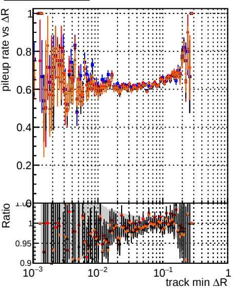
Legend: DOM original4 DOM testIMKFit_initialStepReso DOM testIMKFit_initialStepReso_testSorting
