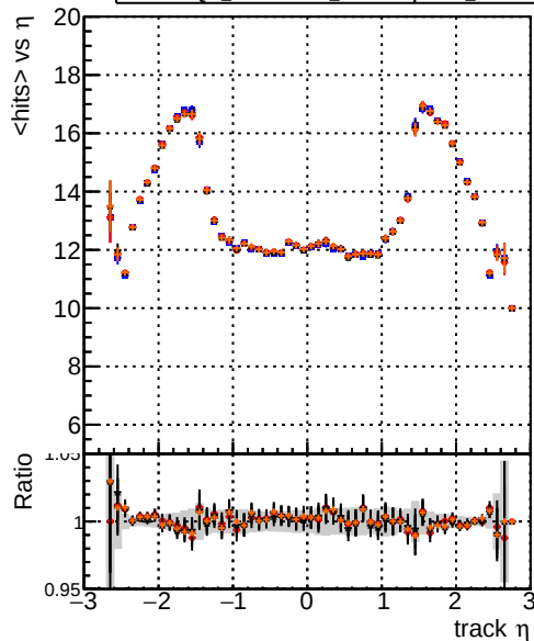
mean hits vs \eta Legend: DQM_original4 (blue line), DQM_testMkFit_initialStepReso (red line), DQM_testMkFitFit_initialStepReso (black line), DQM_testMkFitFit_initialStepReso_testSorting (orange line)
