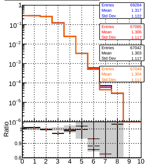
mean hits vs \eta Legend: DQM_original4 (blue line), DQM_testMkFit_initialStepReso (red line), DQM_testMkFitFit_initialStepReso (black line), DQM_testMkFitFit_initialStepReso_testSorting (orange line)
