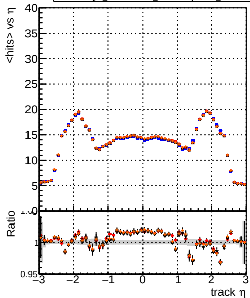
mean hit DQM_testMkFit_initialStepReso DQM_testMkFitFit_initialStepReso DQM_testMkFitFit_initialStepReso_testSorting
