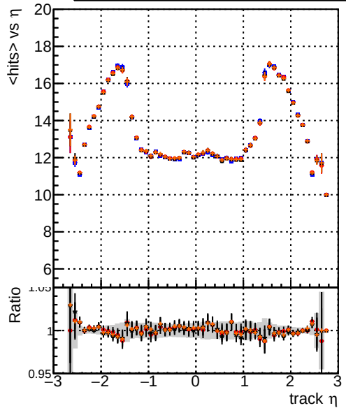
DQM_original4 DQM_testMkFit_fit_initialStepReso DQM_testMkFitFit_initialStepReso DQM_testMkFitFit_initialStepReso_testSorting mean hits
