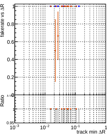
Fake rate vs \Delta R(\text{track, jet}) Legend: DOM original DOM initialStepReso DOM testMKFit DOM testMKFit initialStepReso DOM testMKFit initialStepReso testSorting
