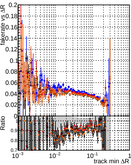
Fake rate vs \Delta R(\text{track, jet}) Legend: - blue squares: original - red circles: testIMKFit - black circles: testIMKFit initialStepReso - orange circles: testIMKFit initialStepReso testSorting
