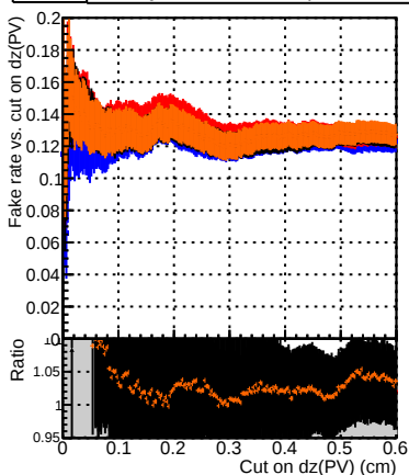
—●— DQM_testMkFitFit_initialStepReso —●— DQM_testMkFitFit_initialStepReso_testSorting
