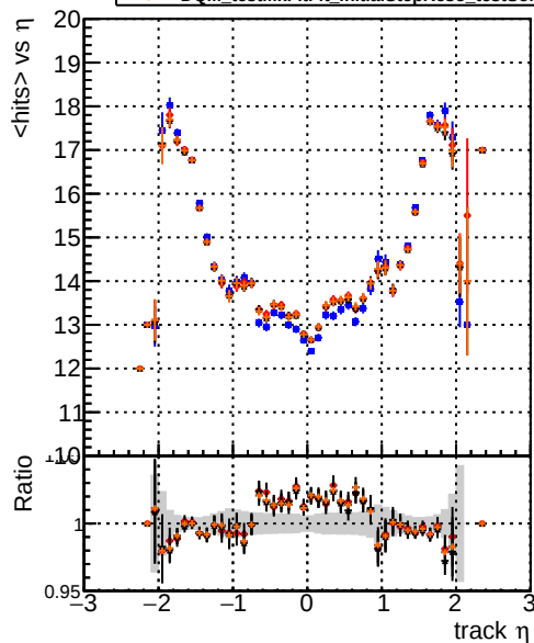
mean hits DQM_testMkFitFit_initialStepReso DQM_testMkFitFit_initialStepReso_testSorting DQM_testMkFitFit_initialStepReso
