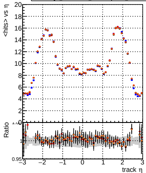
mean hit DQM_testMkFit_initialStepReso DQM_testMkFitFit_initialStepReso DQM_testMkFitFit_initialStepReso_testSorting
