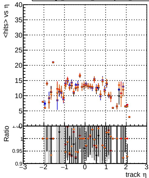
— DQM_original4 — DQM_testMkFit_fit_initialStepReso — DQM_testMkFitFit_initialStepReso — DQM_testMkFitFit_initialStepReso_testSorting mean hits
