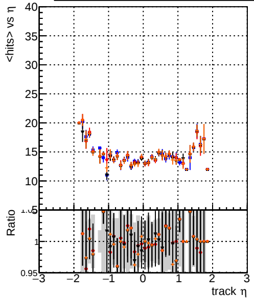
mean hit DQM_original4 DQM_testMkFit_initialStepReso DQM_testMkFitFit_initialStepReso DQM_testMkFitFit_initialStepReso_testSorting
