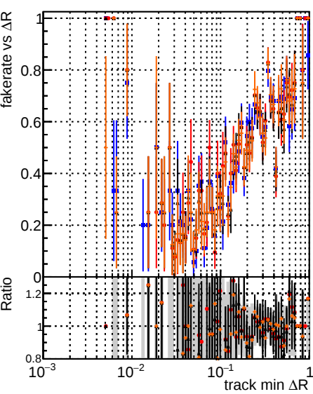
Fake rate vs \Delta R(\text{track, jet}) Legend: DOM original4 DOM testIMKFit initialStepReso DOM testIMKFit initialStepReso testSorting
