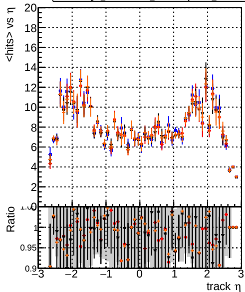
mean hit DQM_testMkFitFit_initialStepReso DQM_testMkFitFit_initialStepReso DQM_testMkFitFit_initialStepReso_testSorting
