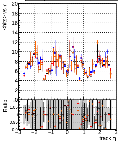
— DQM_original4 — DQM_testMkFit_initialStepReso — DQM_testMkFitFit_initialStepReso — DQM_testMkFitFit_initialStepReso_testSorting mean hit
