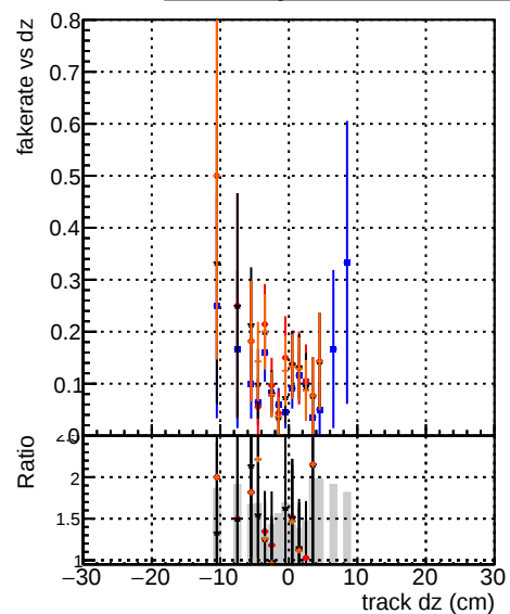
Fake rate vs dz Legend: DOM original4 DOM testMKFit_InitialStepReso DOM testMKFit_InitialStepReso DOM testMKFit_InitialStepReso testSorting
