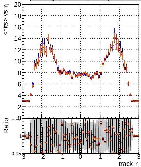
mean hit DQM_origina4 DQM_testMkFit_initialStepReso DQM_testMkFitFit_initialStepReso DQM_testMkFitFit_initialStepReso_testSorting
