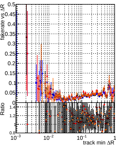
Fake rate vs \Delta R(\text{track, jet}) Legend: DOM original (blue squares) DOM test (red circles) DOM testMKFit initialStepReso (black triangles) DOM testMKFit initialStepReso testSorting (orange diamonds)
