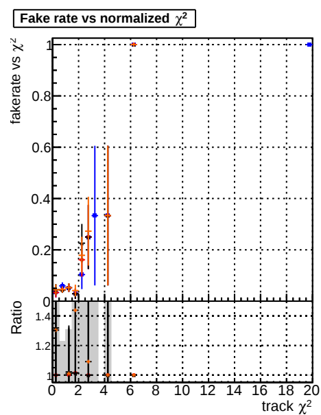
Fake rate vs. \chi^2 Legend: DOM original DOM testMKFit DOM testMKFit-InitialStepReso DOM testMKFit-InitialStepReso testSorting
