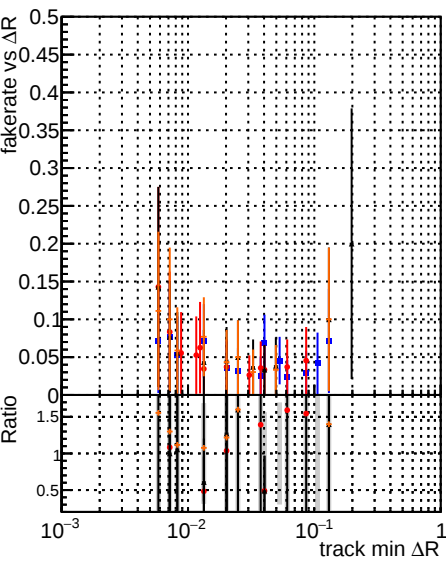
Fake rate vs \Delta R(\text{track, jet}) Legend: DOM original (blue squares) DOM test (red circles) DOM IMKFit initialStepReso (black circles) DOM IMKFit initialStepReso testSorting (orange circles)
