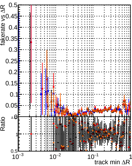
Fake rate vs \Delta R(\text{track, jet}) Legend: DOM original (blue squares) DOM test (red circles) DOM testIMKFit (black triangles) DOM testIMKFit initialStepReso (orange diamonds) testSorting
