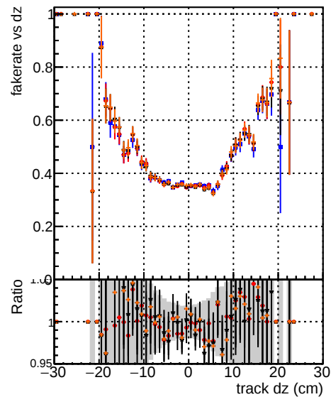
Fake rate vs dz Duplicates Rate vs Dxy Pileup rate vs dxy DCM original4 testMRFit-InitialStepReso testMRFit-InitialStepReso testMRFit-InitialStepReso testSorting
