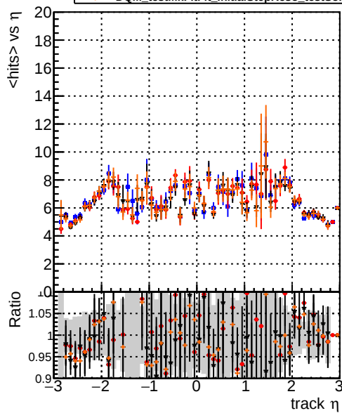
— DQM_original — DQM_testMkFit_initialStepReso — DQM_testMkFitFit_initialStepReso — DQM_testMkFitFit_initialStepReso_testSorting mean hits
