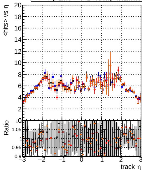
mean hits vs \eta DQM_original DQM_testMkFit_initialStepReso DQM_testMkFitFit_initialStepReso DQM_testMkFitFit_initialStepReso_testSorting
