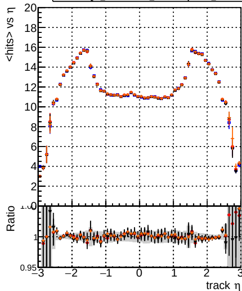
mean hits vs \eta Legend: Blue line: DQM_original4 Red line: DQM_testMkFit_initialStepReso Black line: DQM_testMkFitFit_initialStepReso Orange line: DQM_testMkFitFit_initialStepReso_testSorting
