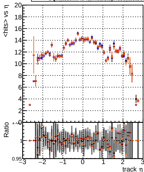
Legend for mean hits vs \eta : Blue line: DQM_original4 Red line: DQM_testMkFit_initialStepReso Black line: DQM_testMkFitFit_initialStepReso Orange line: DQM_testMkFitFit_initialStepReso_testSorting
