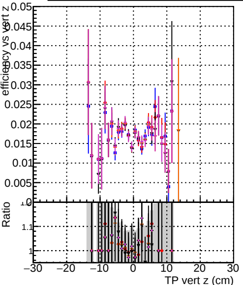
Efficiency vs vertpos Legend: DOM originals DOM testMkFit initialStepReso DOM testMkFit initialStepReso test100 DOM testMkFit initialStepReso test100bf
