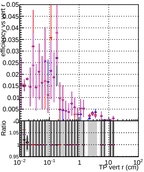
Efficiency vs vertpos Legend: DOM originals DOM testMkFit initialStepReso DOM testMkFit initialStepReso test100 DOM testMkFit initialStepReso test100bf
