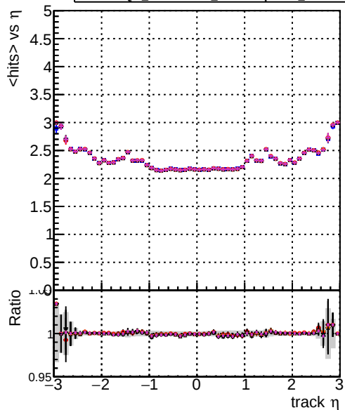
Legend for mean hits vs \eta : DOM originals DOM testMKFit initialStepReso DOM testMKFit initialStepReso test100 DOM testMKFit initialStepReso test100bfb
