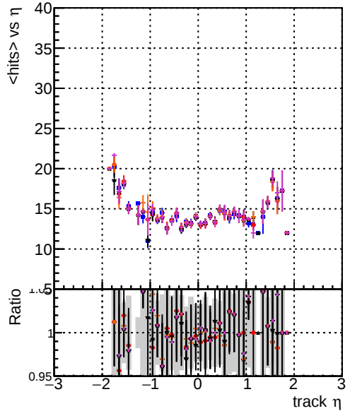
mean hits vs \eta — DQM original — DQM testMkFit initialStepReso — DQM testMkFit initialStepReso test100 — DQM testMkFit initialStepReso test100bfb
