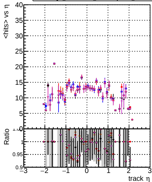
DQM original DQM testMkFit initialStepReso DQM testMkFit initialStepReso test100 DQM testMkFit initialStepReso test100bfbf mean hits
