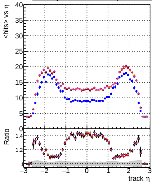
Legend: DQM original, DQM testMkFit initialStepReso, DQM testMkFit initialStepReso test100bf, DQM testMkFit initialStepReso test100bf mean hits
