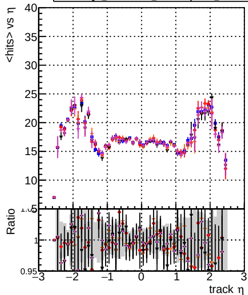
DOM originals DOM testMkFit initialStepReso DOM testMkFit initialStepReso test100b DOM testMkFit initialStepReso test100b mean hits
