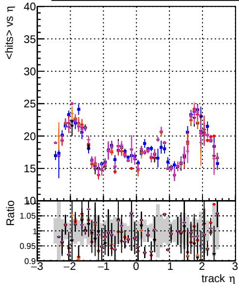
mean hits vs \eta Legend: DOM originals (blue), DOM testMkFit initialStepReso (red), DOM testMkFit initialStepReso test100 (orange), DOM testMkFit initialStepReso test100b (purple)
