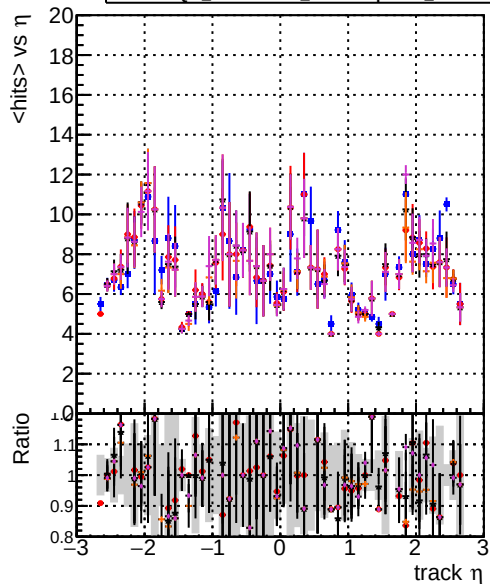
Legend: DQM originals, DQM testMkFit initialStepReso, DQM testMkFit initialStepReso test100, DQM testMkFit initialStepReso test100b mean hits
