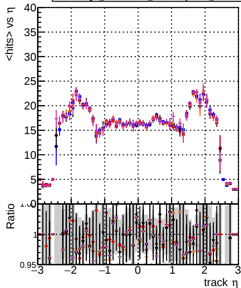
Legend: — DQM original — DQM testMkFit initialStepReso — DQM testMkFit initialStepReso test100bf — DQM testMkFit initialStepReso test100bf
