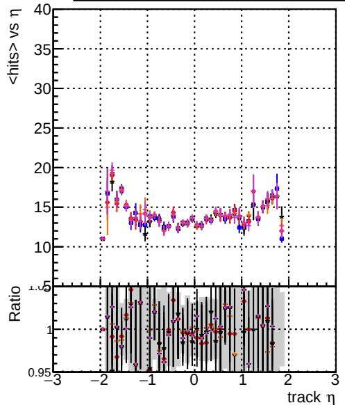
mean hit DQM originals DQM testMkFit initialStepReso DQM testMkFit initialStepReso test100 DQM testMkFit initialStepReso test100bf
