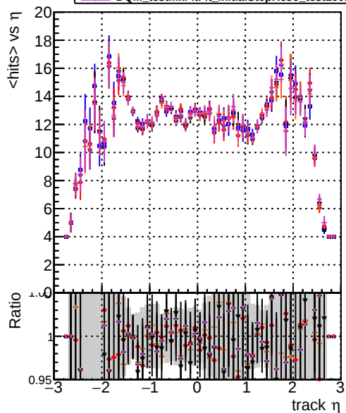
mean hits vs \eta Legend: - DQM originals - DQM testMkFit initialStepReso - DQM testMkFit initialStepReso test100 - DQM testMkFit initialStepReso test100bf
