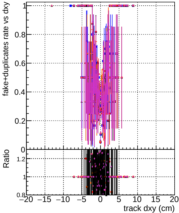
DQM_original4 DQM_testMkFit_initialStepReso DQM_testMkFitFit_initialStepReso DQM_testMkFitFit_initialStepReso_test100 DQM_testMkFitFit_initialStepReso_test100bf
