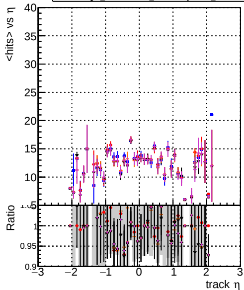
Legend for mean hits vs \eta : DOM originals testMkFit initialStepReso testMkFit initialStepReso test100 testMkFit initialStepReso test100bf testMkFit initialStepReso test100bf
