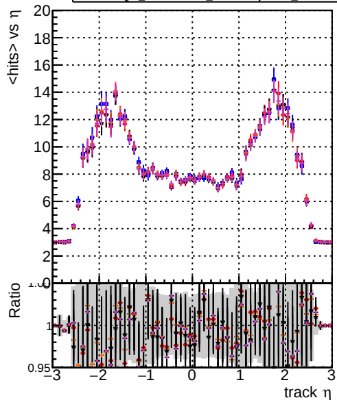
mean hit DQM original DQM testMkFit initialStepReso DQM testMkFit initialStepReso test100 DQM testMkFit initialStepReso test100bf
