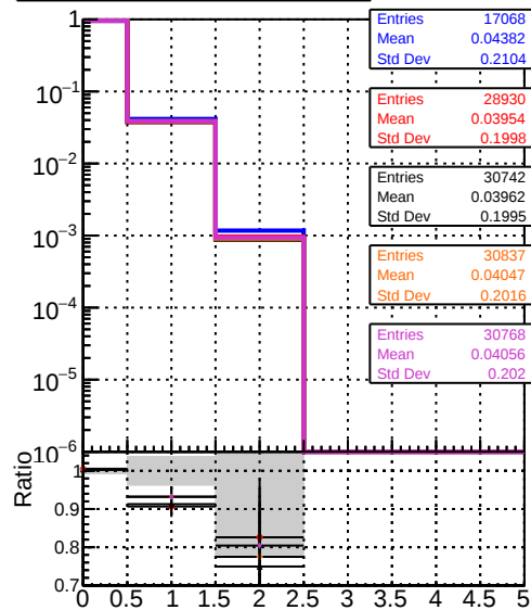
Legend: DQM originals, DQM testMkFit initialStepReso, DQM testMkFit initialStepReso test100, DQM testMkFit initialStepReso test100bf mean hit
