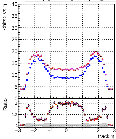
Legend: DQM originals, DQM testMkFit initialStepReso, DQM testMkFit initialStepReso test100, DQM testMkFit initialStepReso test100bf mean hit
