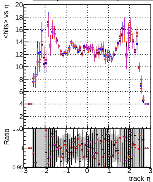
mean hits vs \eta Legend: DQM originals, DQM testMkFit initialStepReso, DQM testMkFit initialStepReso test100, DQM testMkFit initialStepReso test100bf
