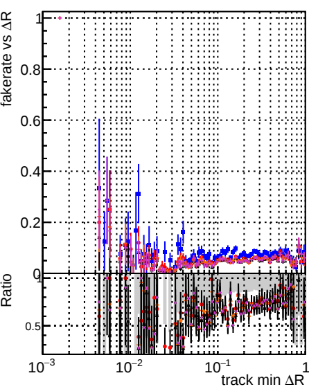
Fake rate vs \Delta R(\text{track, jet}) DQM original4 InitialStepReso test100br
