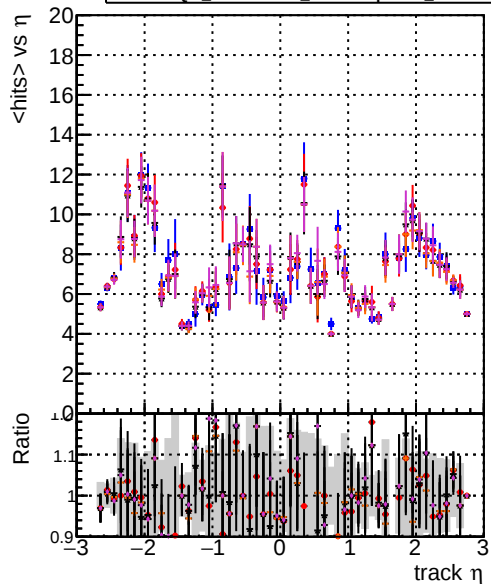
mean hit DOM originals DOM testMkFit initialStepReso DOM testMkFit initialStepReso test100 DOM testMkFit initialStepReso test100bfr
