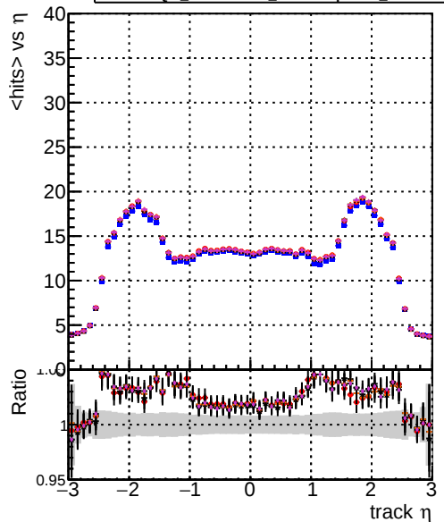
DQM originals testIMkFit initialStepReso DQM testIMkFit initialStepReso DQM testIMkFit initialStepReso test100 DQM testIMkFit initialStepReso test100bf mean hits
