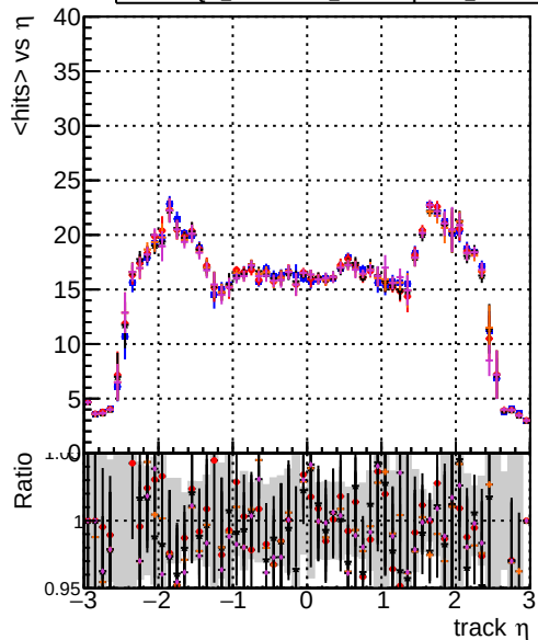
DQM originals DQM testMKFit initialStepReso DQM testMKFit initialStepReso test100 DQM testMKFit initialStepReso test100b mean hit
