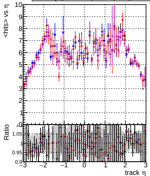
mean hits vs \eta DOM originals DOM testMkFit initialStepReso DOM testMkFit initialStepReso test100bf DOM testMkFit initialStepReso test100bf
