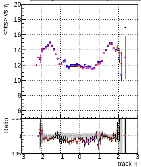
Legend: DQM originals, DQM testMkFit initialStepReso, DQM testMkFit initialStepReso test100, DQM testMkFit initialStepReso test100bfb mean hits
