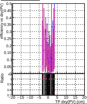
Efficiency vs Dxy(PV) Legend: DOM_original4 DOM_testMkFit_initialStepReso DOM_testMkFitFit_initialStepReso DOM_testMkFitFit_initialStepReso_test100 DOM_testMkFitFit_initialStepReso_test100bf
